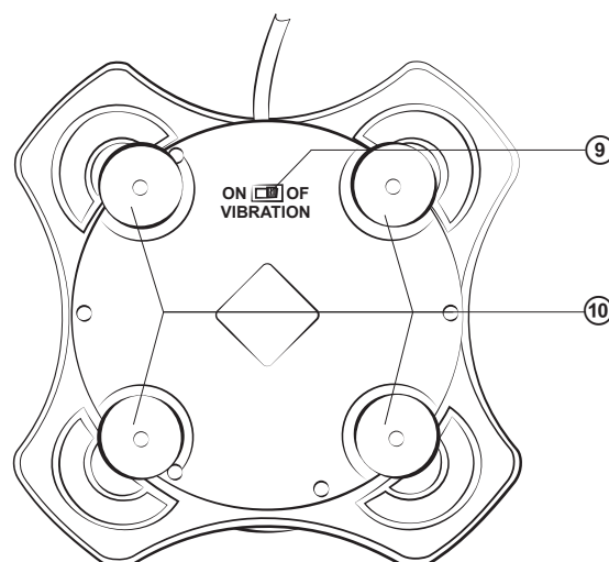
Fig. 3. Bottom view
